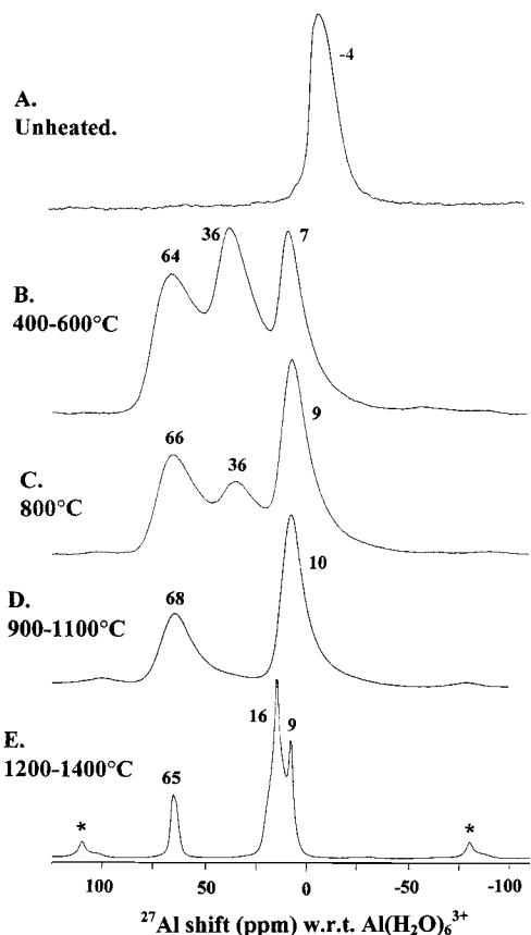
Fig. 6. ^{27}\text{Al} MAS NMR spectra of citrate-derived CA6 gel, unheated and heated at the indicated temperatures.
