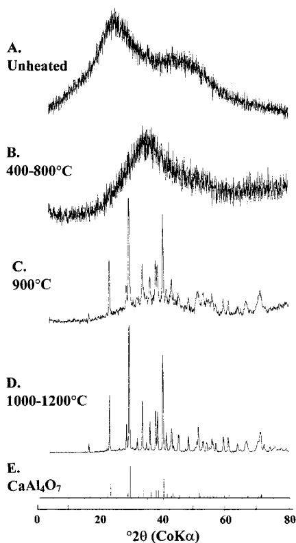
Fig. 2. X-ray powder diffractograms of CA2 citrate-derived gel for: (A) unheated; (B) 400–800°C; (C) 900°C; (D) 1000–1200°C heated for 60 min; (E) CaAl 4 O 7 diffraction pattern (PDF no. 23-1037).
